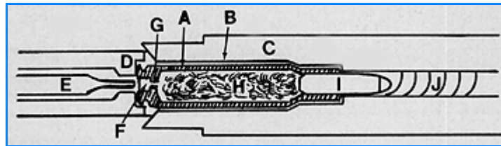
FIG. 36-5 A schematic view of the components of a cartridge contained within the solid steel envelope formed by the barrel and breeching mechanism of the typical rifle.
